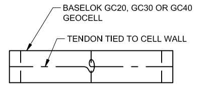
DETAIL "1"
