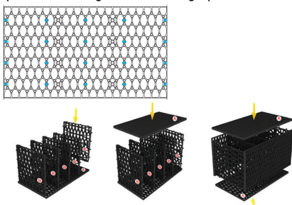
Figure 2: Follow these steps to assemble the underdrain units
