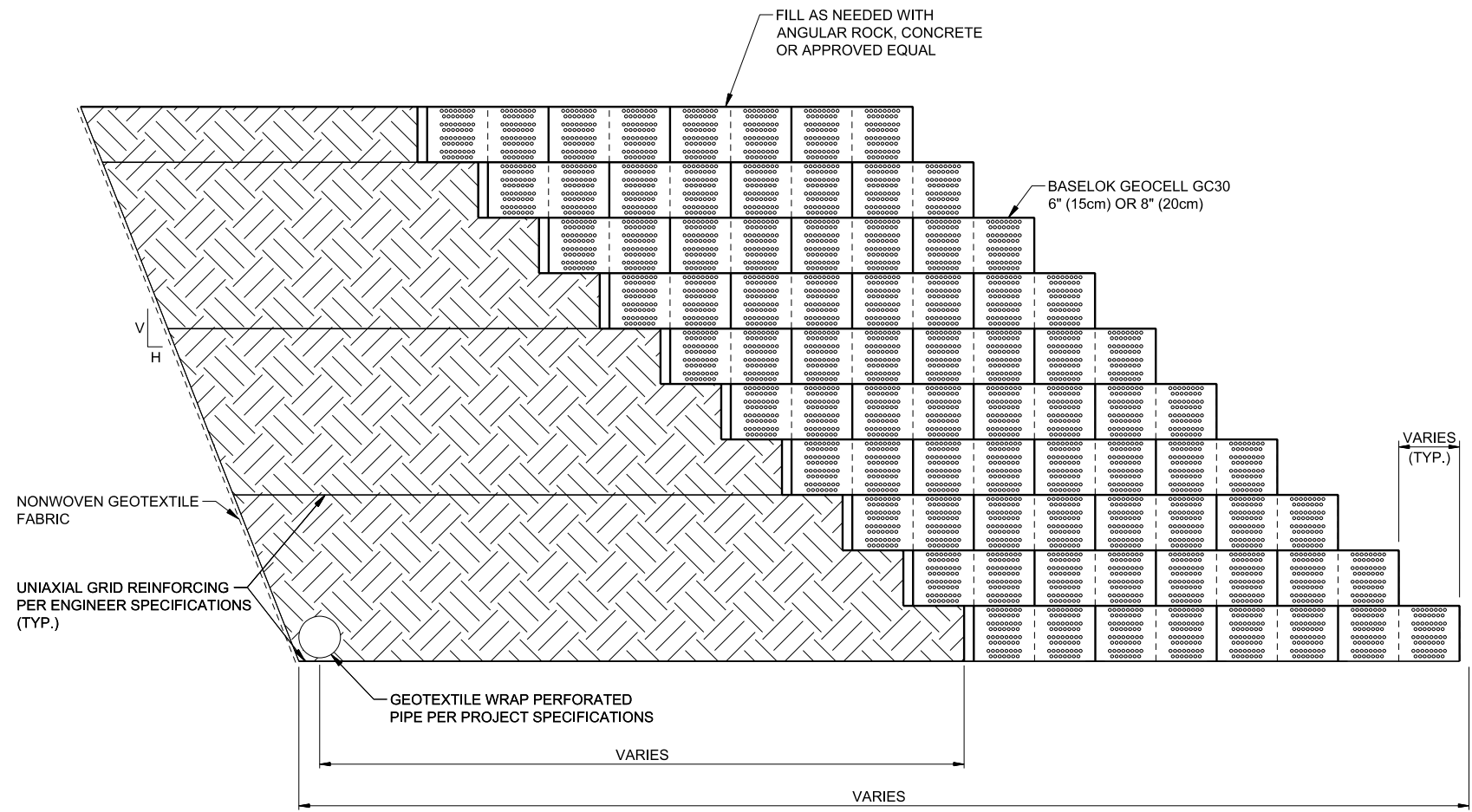
BASELOK GEOCELL RETAINING WALL - 4 CELL EMBEDMENT
