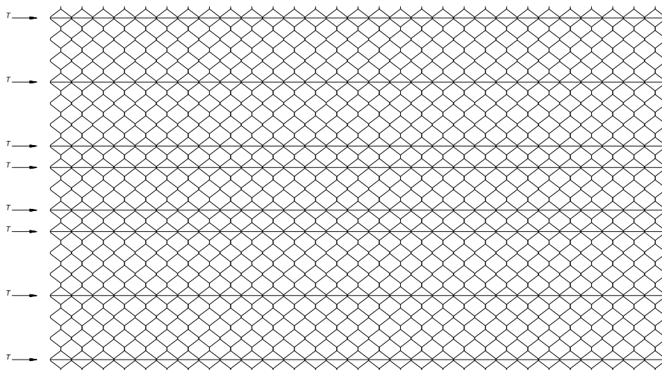
GEOCELL GC30W (8) TENDON LAYOUT
